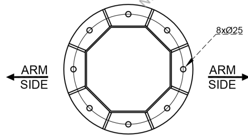
BASE PLATE
